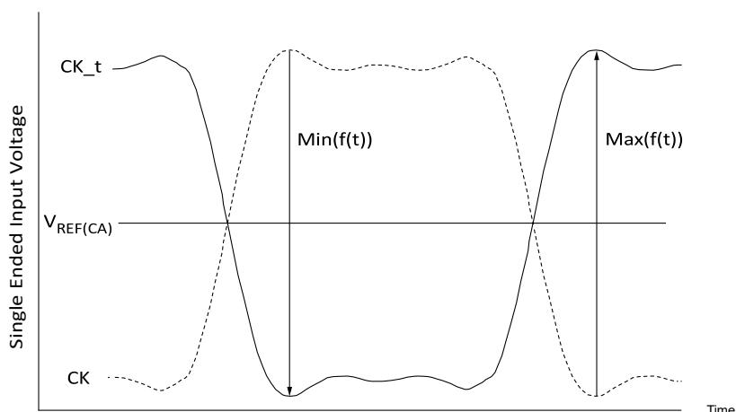
Figure 13-Definition of Differential Clock Peak Voltage
