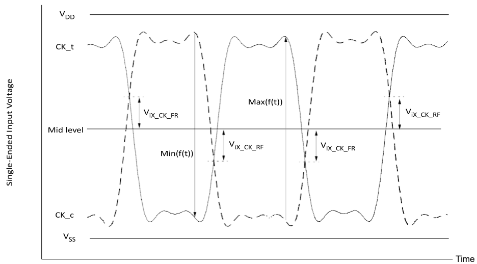
Figure 16-VixDefinition (Clock)
