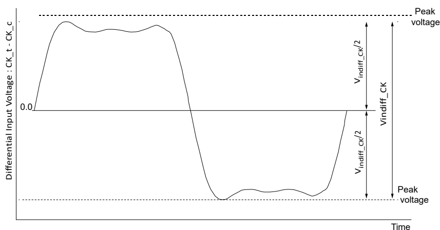
Figure 12-CK Differential Input Voltage
