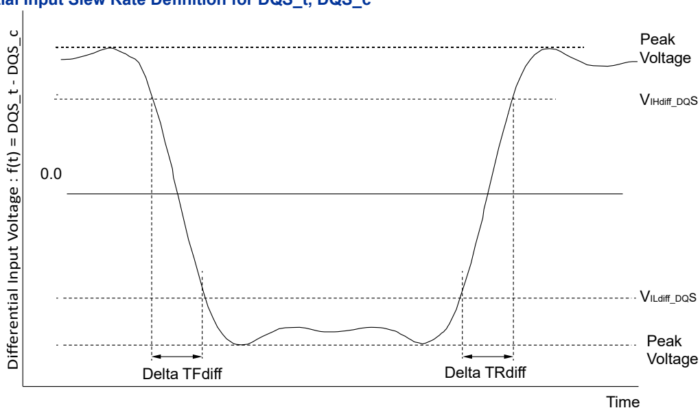
Figure 20-Differential Input Slew Rate Definition for DQS t , DQS c
