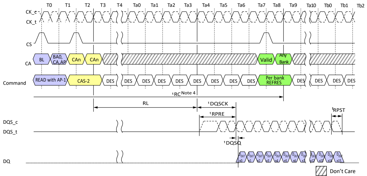
Figure 10-Burst READ With AUTO PRECHARGE Operation Followed by Per-Bank Refresh
