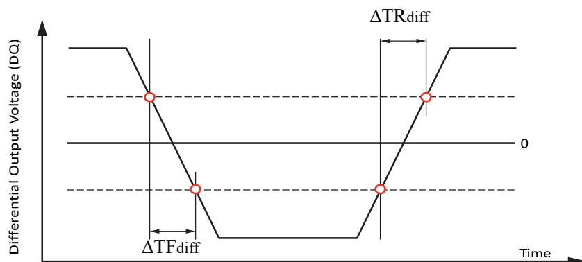
Figure 23-Differential Output Slew Rate Definition
