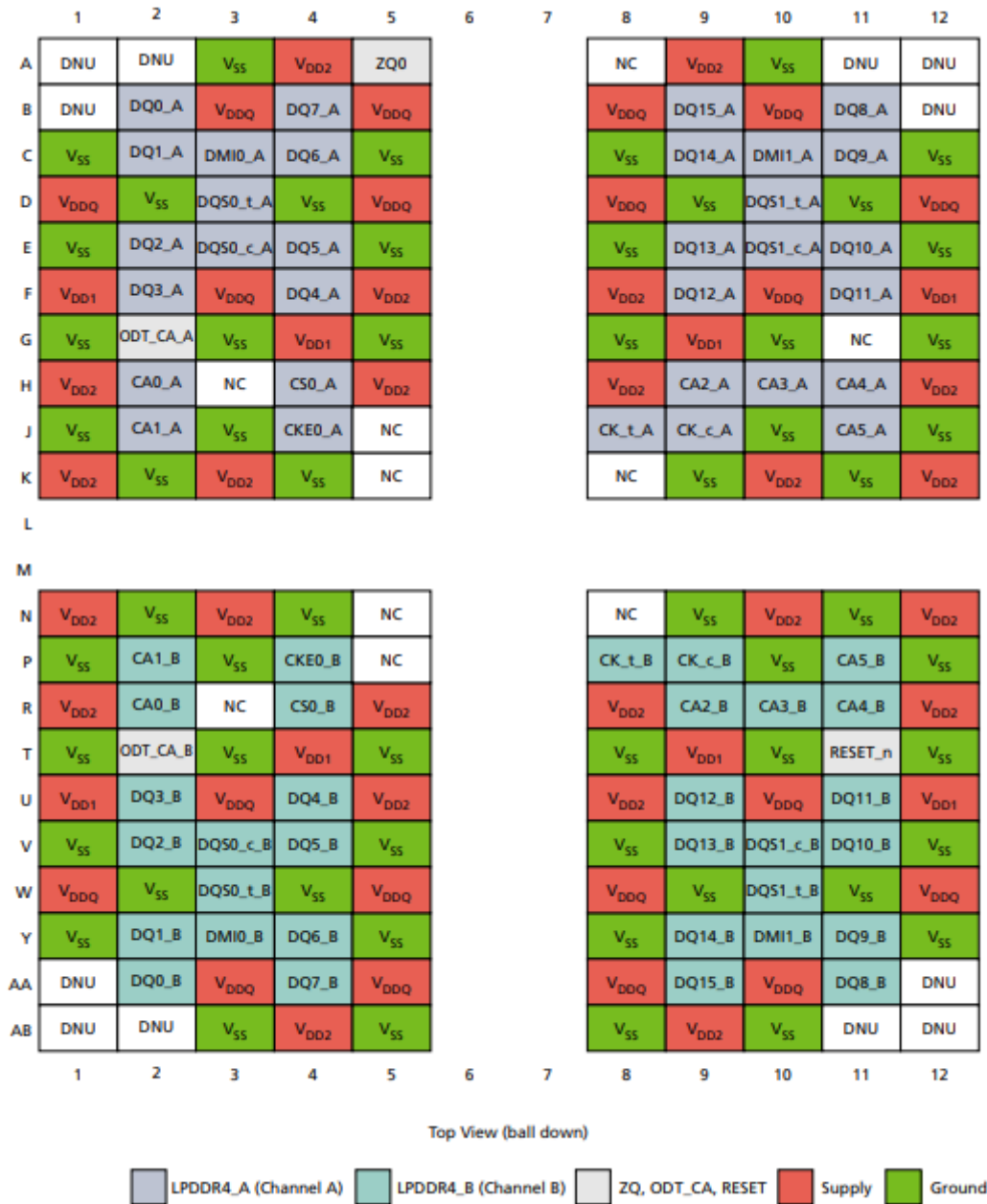
Figure 2- 200-Ball Dual-Channel, Single-Rank Discrete FBGA
