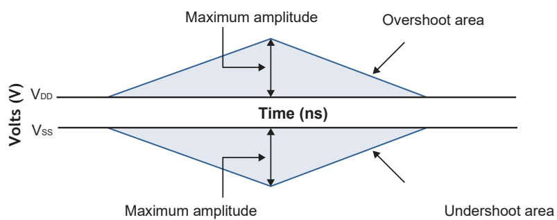
Figure 24-Overshoot and Undershoot Definition
