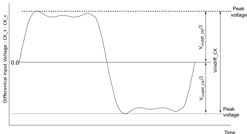
Figure 12-CK Differential Input Voltage
