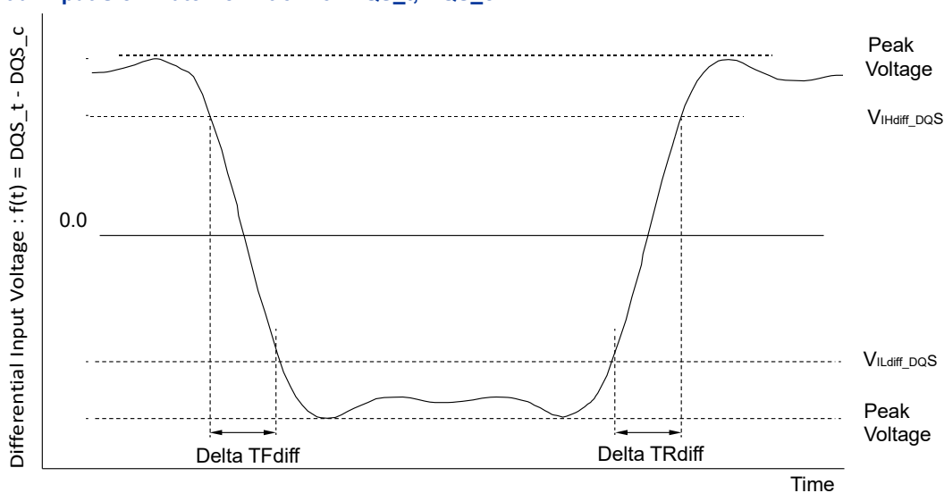
Figure 20-Differential Input Slew Rate Definition for DQS_t, DQS_c
