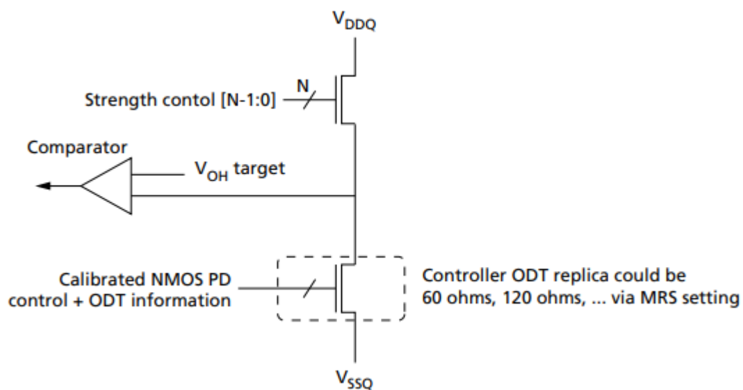
Figure 27- Pull-Up Calibration
