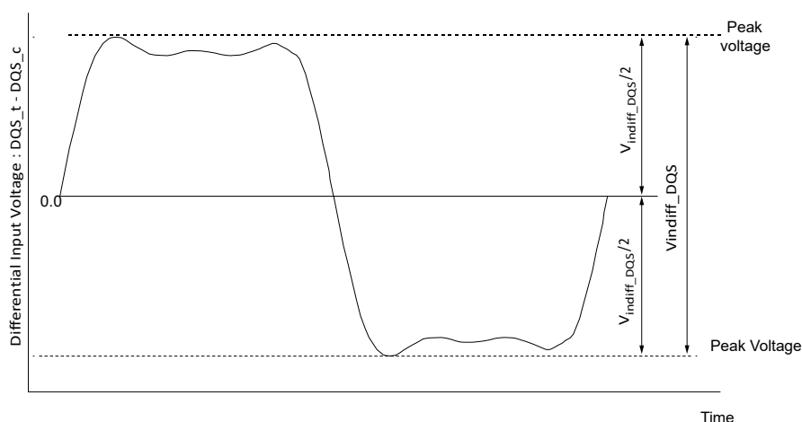
Figure 17-DQS Differential Input Voltage
