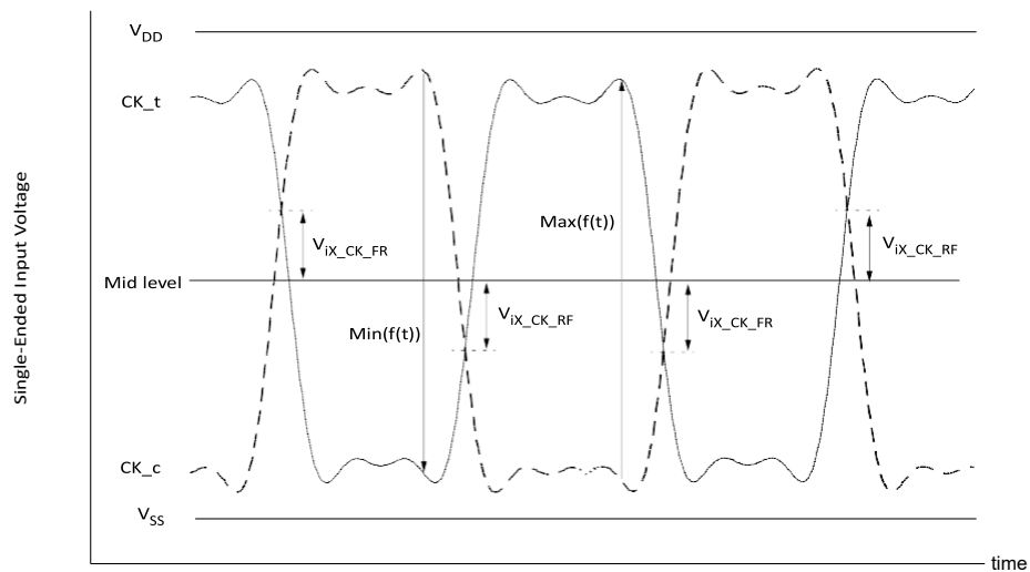
Figure 16-VixDefinition (Clock)
