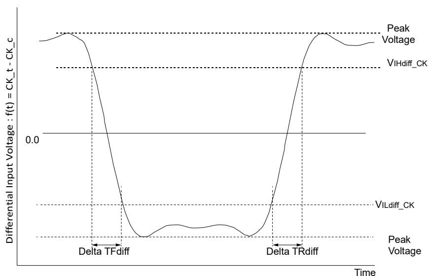
Figure 15-Differential Input Slew Rate Definition for CK_t, CK_c
