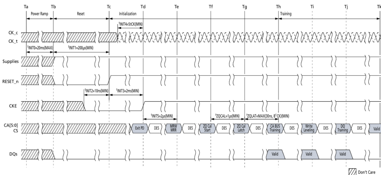
Figure 4-Voltage Ramp and Initialization Sequence
