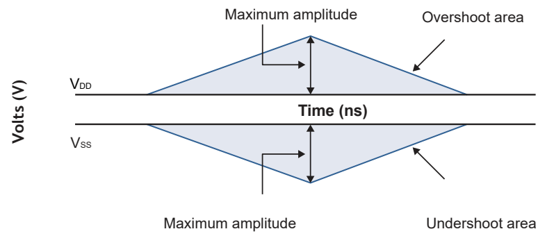
Figure 24-Overshoot and Undershoot Definition
