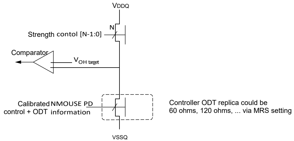
Figure 27- Pull-Up Calibration
