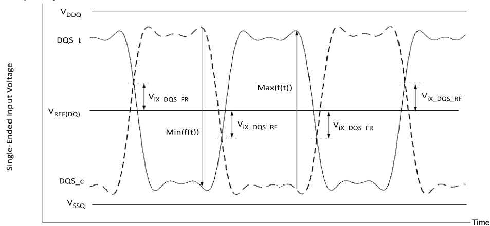
Figure 21- VixDefinition (DQS)
