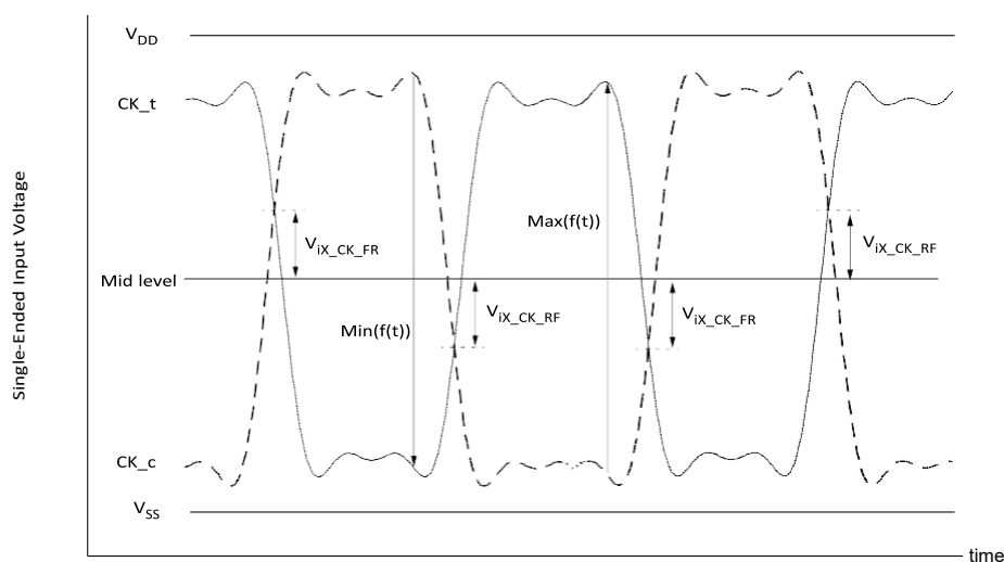
Figure 16-VixDefinition (Clock)
