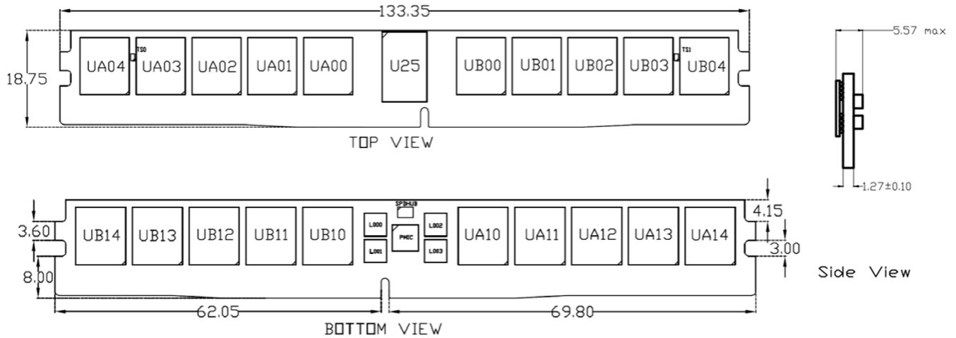
Figure 2 - Package Dimensions_SCA32GR13H1F1V-56B
