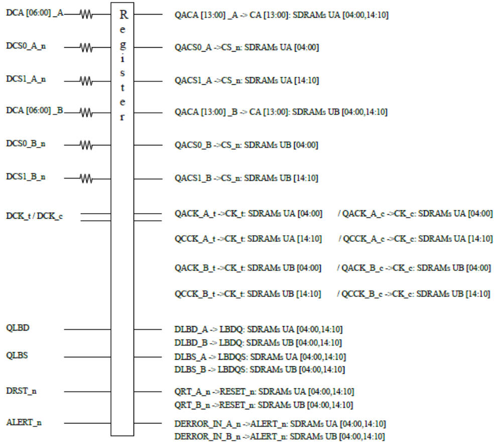
Figure 1 - Function Block Diagram_SCA32GR13H1F1V-56B
