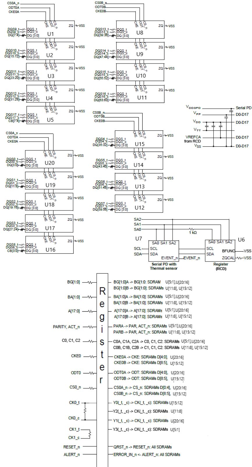
Figure 1 - Function Block Diagram_SCC32GP02C3F1V-32AA
