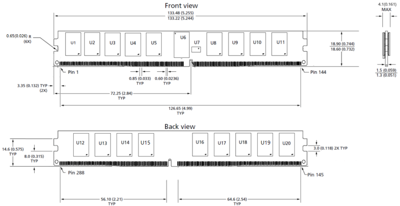
Figure 2 - Package Dimensions_SCC32GP02C3F1V-32AA
