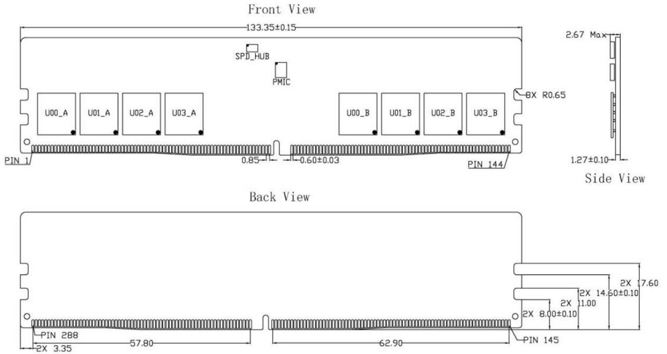
Figure 2 - Package Dimensions_UCA16GU03A3F1C-56B
