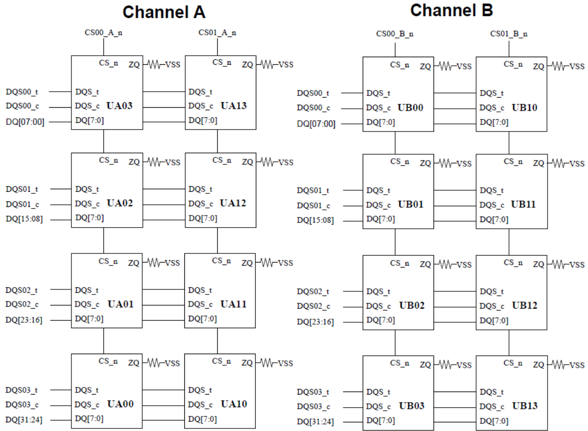
Figure 1 - Function Block Diagram_SCA32GU13C2F1C-48B
