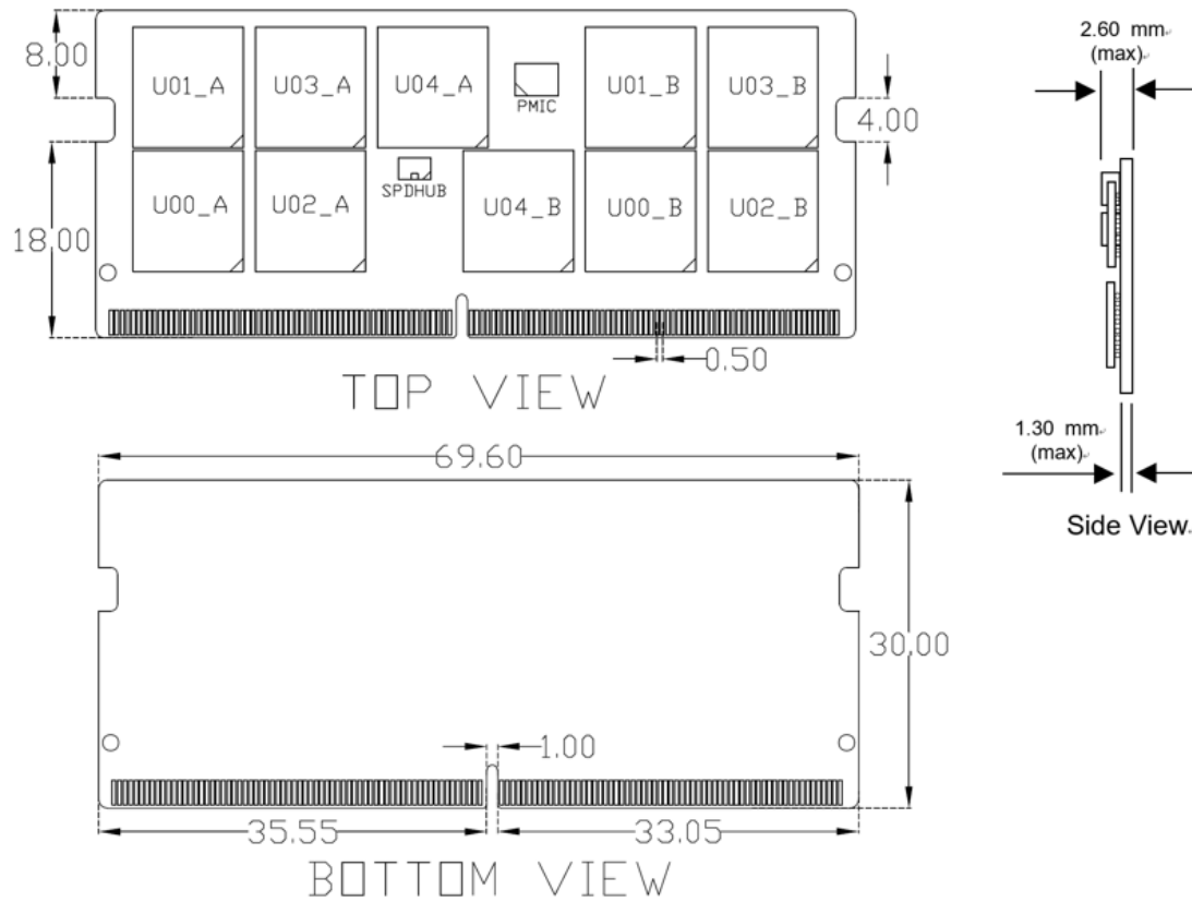
Figure 2 - Package Dimensions_SCA16GT03H1F1C-56B
