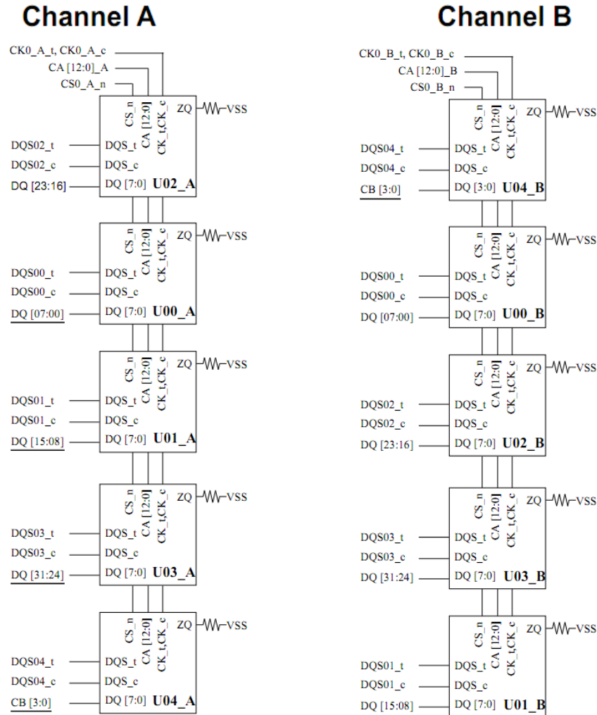
Figure 1 - Function Block Diagram_SCA16GT03H1F1C-56B
