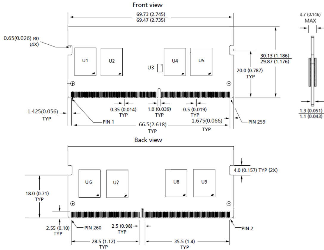
Figure 2 - Package Dimensions_SCC16GX03C3F1C-32AA
