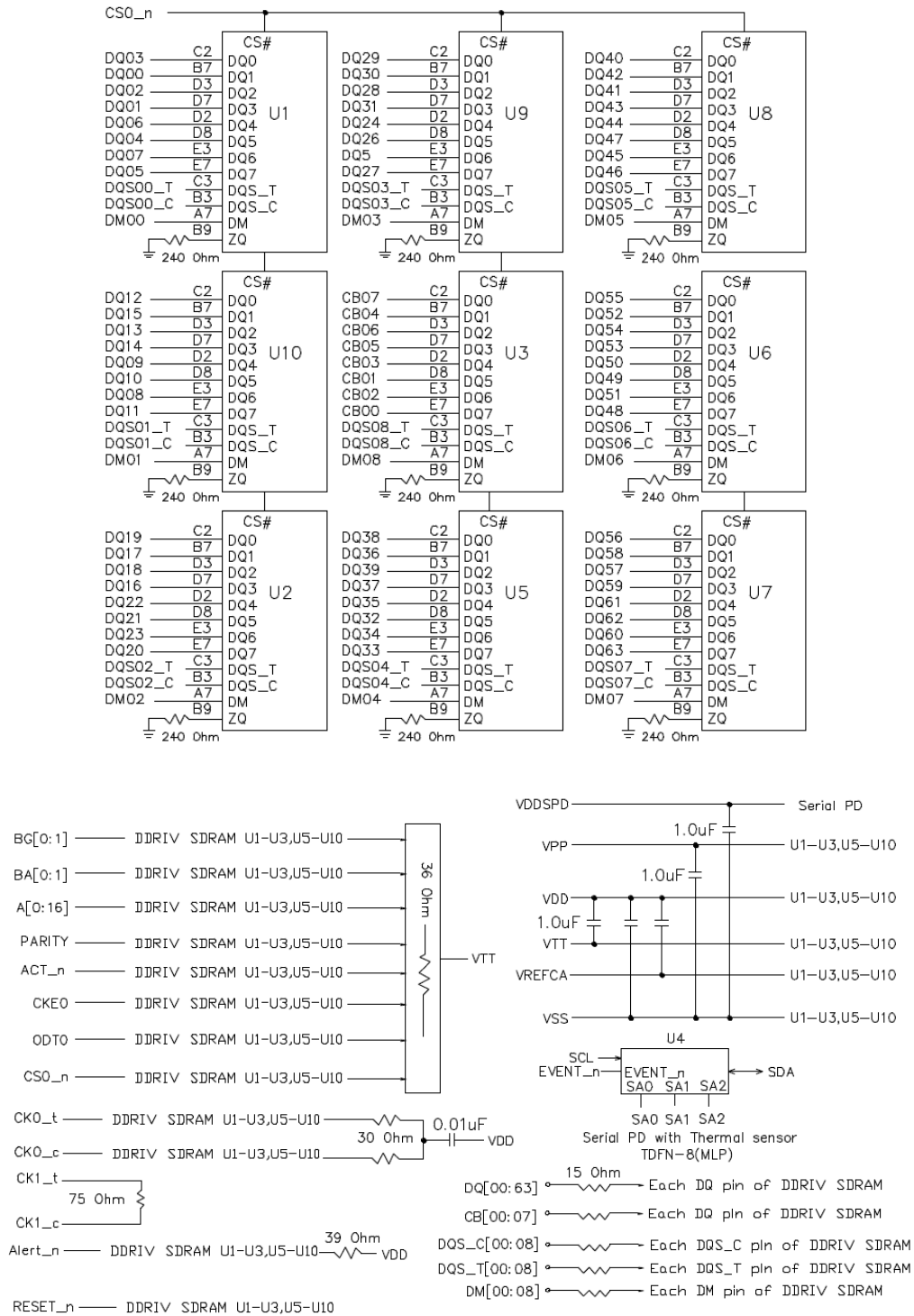
Figure 1 - Function Block Diagram_SCC16GX03C3F1C-32AA
