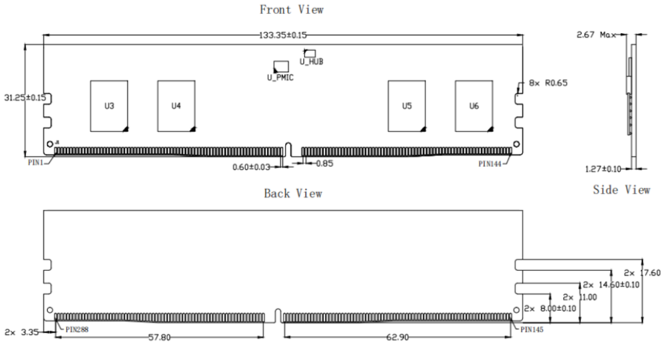
Figure 2 - Package Dimensions_SCA08GU04H1F1C-56B
